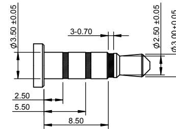
Ø 3.50 mm 4 POLE PLUG DETAIL DRAWING
