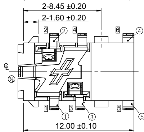
Ø 3.50 mm 4 POLE PLUG DETAIL DRAWING
