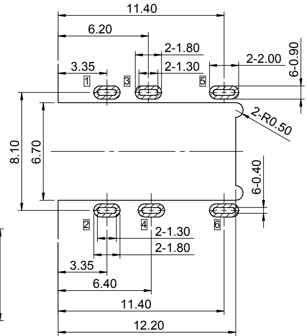
PCB LAYOUT(TOP VIEW) TOLERANCE ±0.05
